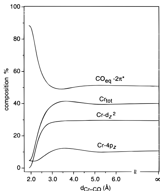
Figure 3. Changes in the composition of the lowest virtual orbital of Cr(CO) 6 along the Cr-CO dissociation coordinate. The orbital is initially the a 1 component (in C 4v symmetry) of the 9t 1u (in O h ) level and evolves into the a 1 LUMO of Cr(CO) 5 . The percentage compositions are derived from a Mulliken population analysis.
