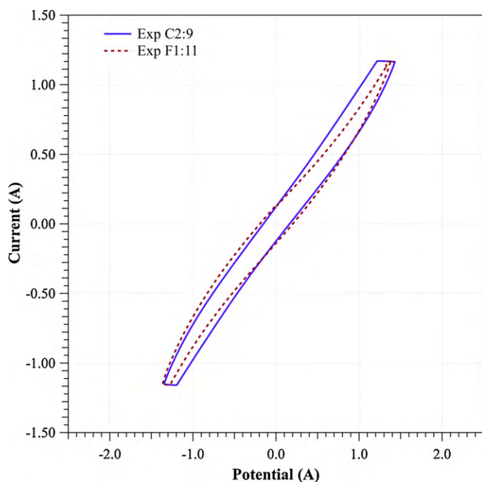
Fig. 4. Cyclic voltammety measurements of Exp C2, Test 9 and Exp F1, Test 11.
