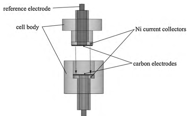
Fig. 2. Schematic view of EDLC cell. Cell body is constructed of Teflon.
