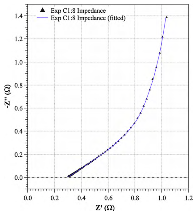
Fig. 6. AC impedance responses for activated carbon electrode in Test 8 of experiment C1. Numerical fitting was based on the equivalent circuit shown in Fig. 4. Most experiments gave similar results except those already noted in the test.
