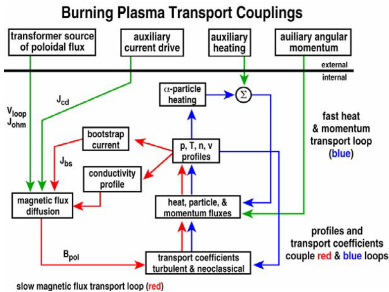
Figure 2.2. Illustration of complex feedback loops and non-linear couplings among basic plasma phenomena that result in the final burning plasma state.
