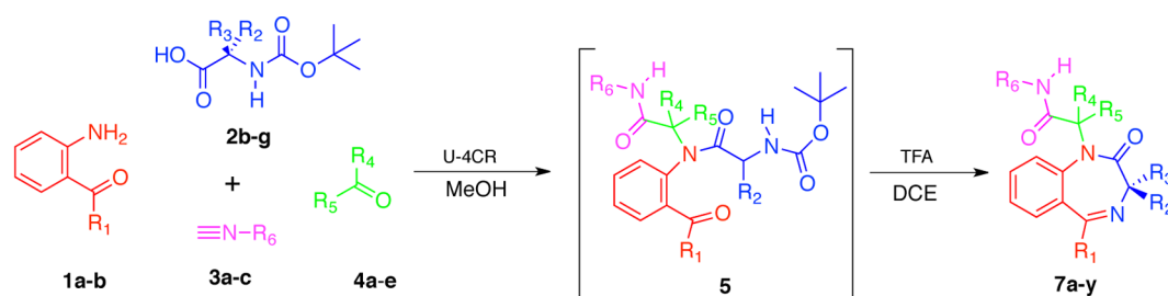
Scheme 3. U-4CR-Based Assembly of Enantiopure BZDs Incorporating Functional and Stereochemically Diverse Groups at Position 3
